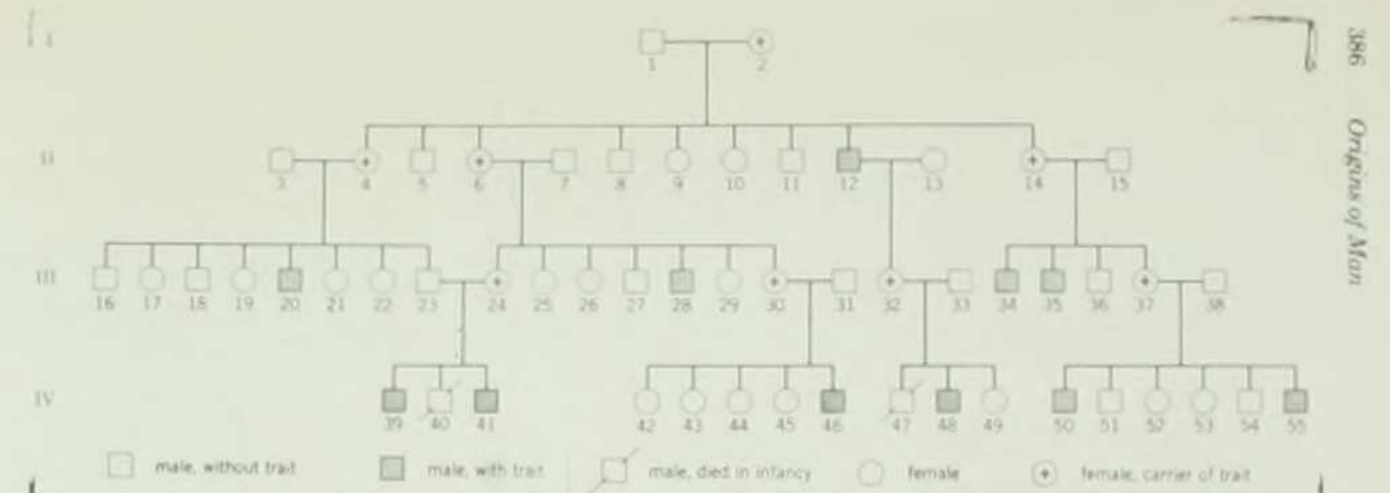
Fig. 23.5. A royal pedigree of hemophilia. Part of the genealogy of royal families of Europe shows the pedigree of hemophilia, a rare X-linked recessive trait. It is presumed that Queen Victoria (2) was the original carrier of the trait in European royal houses. For those readers who are interested in royal lineages, the following individuals are in the pedigree: (1) Prince Albert, (2) Queen Victoria, (3) Frederic III of Germany, (4) Victoria, Princess Royal, (5) Edward VII, (6) Alice, Duchess of Hesse, (7) Louis IV (Ludwig) of Hesse, (8) Alfred, (9) Helena, (10) Louise, (11) Arthur, (12) Leopold, Duke of Albany, (13) Helena of Waldeck and Pyrmont, (14) Beatrix, (15) Henry Maurice of Battenberg, (16) Kaiser Wilhelm II, (17) Charlotte, (18) Sigmund, (19) Victoria, (20) Joachim, (21) Sophie, (22) Margaret, (23) Henry of Prussia, (24) Irene, (25) Victoria, Marchioness of Milford Haven, (26) Elizabeth Fedorovna, (27) Ernst Louis (Ludwig) of Hesse, (28) Frederick William, (29) Marie Victoria, (30) Alice Alexandra, (31) Czar Nicolas II, (32) Alice, Countess of Athlone, (33) Alexander of Teck, Earl of Athlone, (34) Leopold of Mountbatten, (35) Maurice of Battenberg, (36) Alexander of Cambridge, (37) Victoria Eugenie, (38) Alfonso XIII of Spain, (39) Sigmund, (40) Heinrich, (41) Waldemar, (42) Olga, (43) Tatiana, (44) Marie, (45) Anastasia, (46) Czarévitch Alexis, (47) Maurice, (48) Rupert, Viscount Trematon, (49) May Helen, (50) Alfonso Po of Asturias, (51) Jaime, (52) Beatrice, (53) Maria, (54) Joan, (55) Gonzale. Many individuals in Victoria's lineage have been omitted from generations III and IV. For two of the males who died in infancy, (40) and (47), there is no evidence that they either had or did not have the trait.
